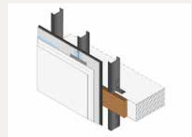
6. Apply base coat and finishing
